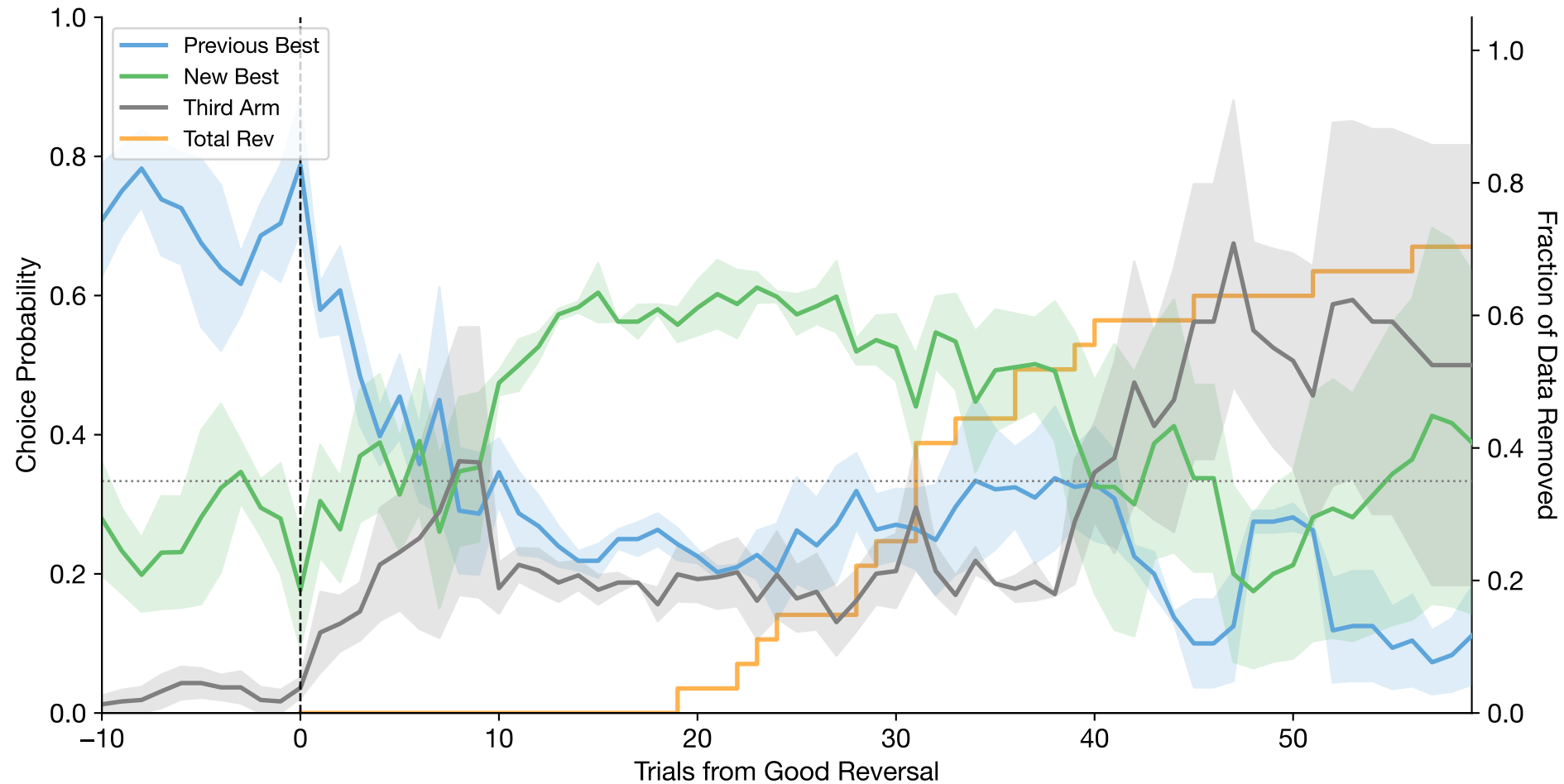
Good Reversal-Aligned Choices (mean \pm se across subjects | n=5 subjects, n=27 reversals)
